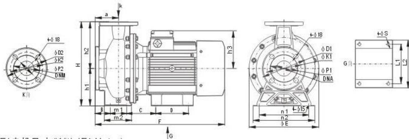
配套IE1电机尺寸 (With IE1 Motor)
