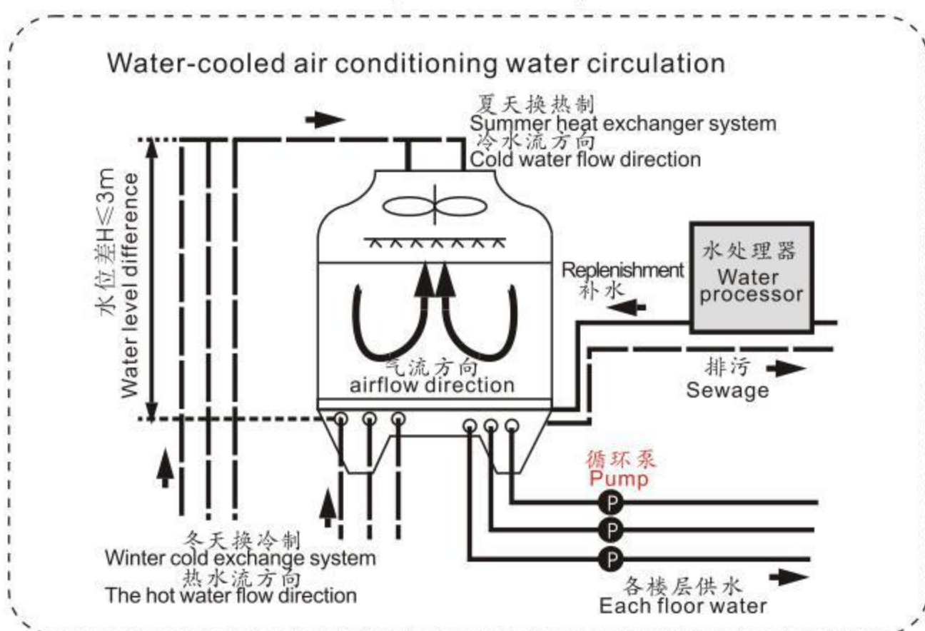
工作原理图 Working principle diagram
