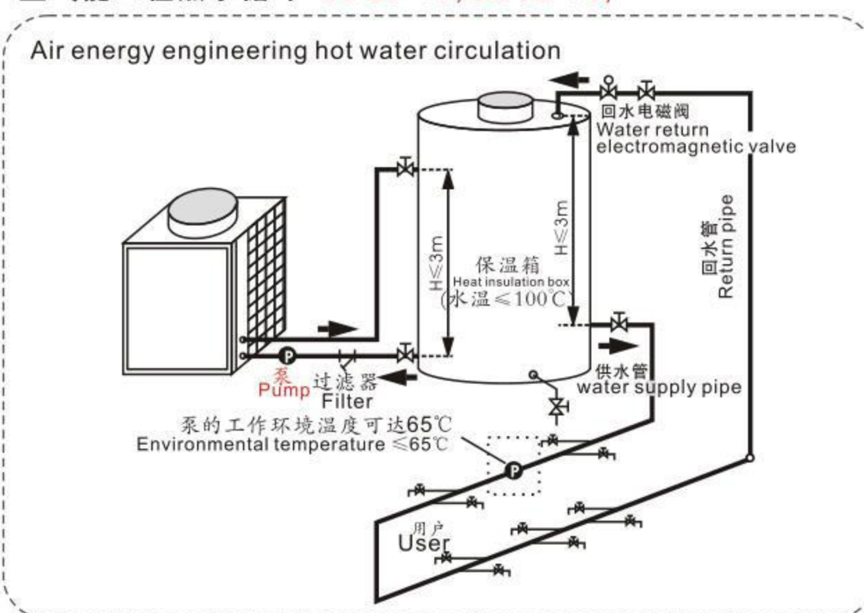
工作原理图 Working principle diagram
